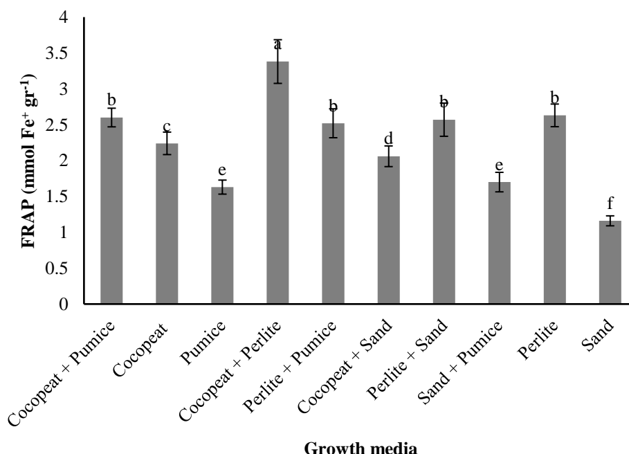
Fig. 15. Simple effects of growth media on FRAP antioxidant activity in O. basilicum . Different letter(s) on the bars showed statistically significant differences ( P < 0.01 ). Error bars represent standard deviation.
