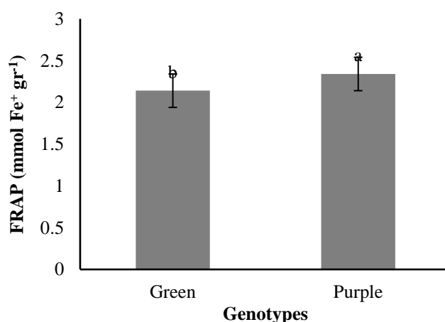
Fig. 14. Simple effects of genotype on FRAP antioxidant activity in O. basilicum . Different letter(s) on the bars showed statistically significant differences ( P < 0.01 ). Error bars represent standard deviation.
