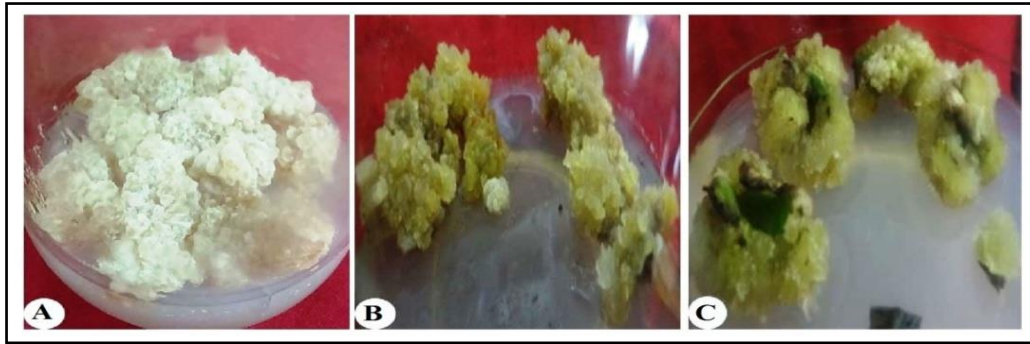
Fig. 1. Induction of callus on MS (Murashige and Skoog) medium supplemented with 5.0 \mu\text{M} NAA(Naphthaleneacetic acid)+ 2.5 \mu\text{M} BAP (6-Benzylaminopurine) + 10% CW (coconut water) using root (A), hypocotyl (B), and cotyledonary leaf (C) explants in S. marianum .
