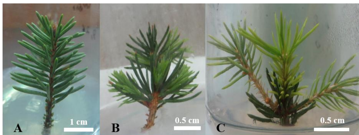
Fig. 1. Shoot proliferation of P. abies micro-cuttings in MS media. Control (A), supplemented with Zeatin (B) and with 2iP (C).
