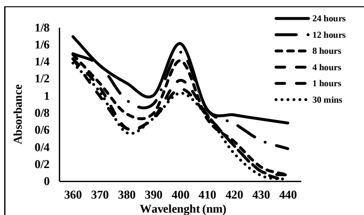
Fig. 3. The absorbance spectrum of silver nanoparticles (AgNPs) synthesized by T. parthenium extract at time intervals.
